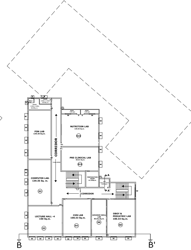
SECOND FLOOR PLAN SCALE :- 1:200
