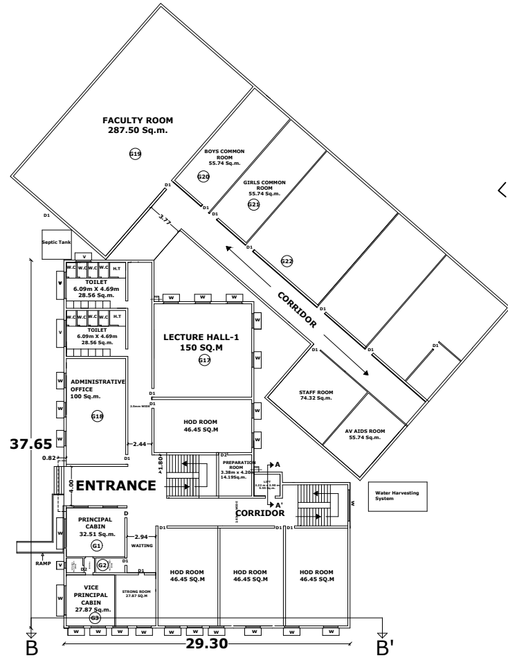
GROUND FLOOR PLAN SCALE :- 1:200
