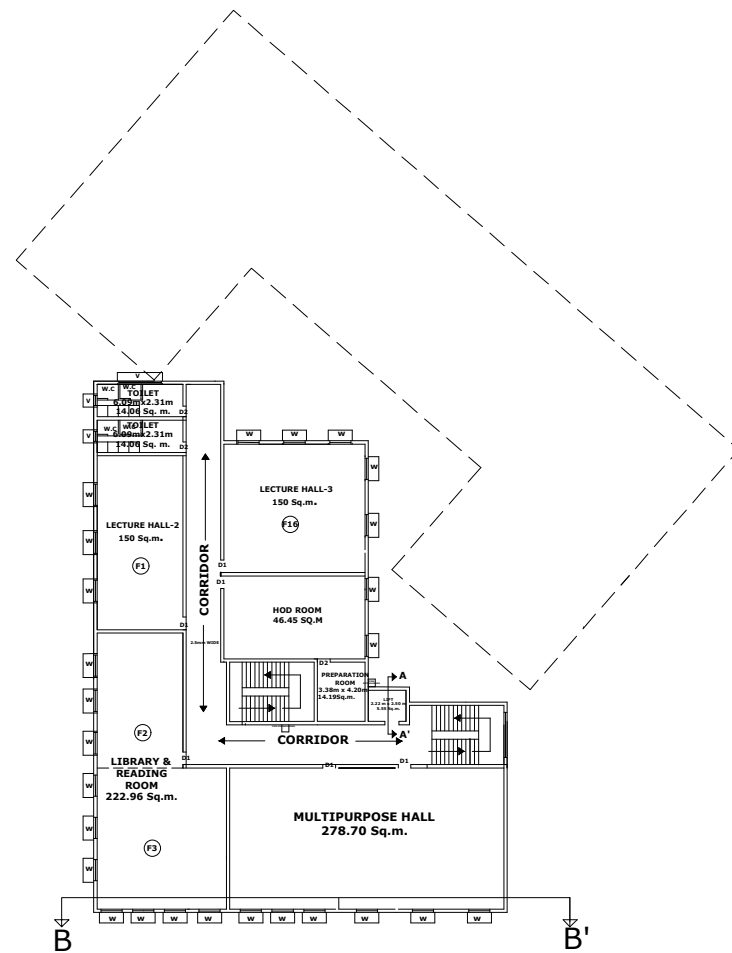
FIRST FLOOR PLAN SCALE :- 1:200
